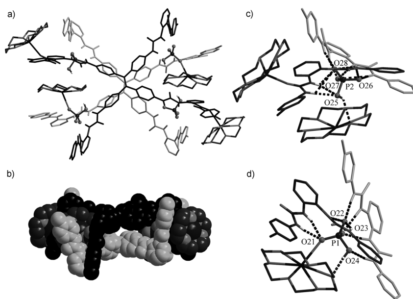
Figure 3. Crystal structure of [(HPO 4 ) 4 ( L 2 ) 2 ] 8- ( 1 ). a) The coordination of four HPO 4 2- ions by two ligands; b) Side view of the space-filling representation; c,d) Hydrogen bonds (broken lines) around the HPO 4 2- ions.
